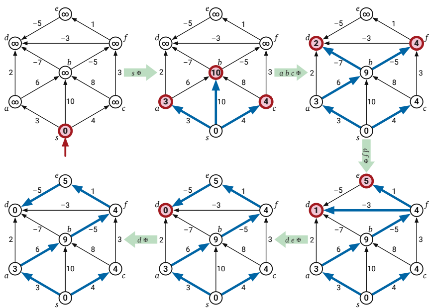
Figure 8.17. A complete run of Moore's algorithm on a directed graph with negative edges. Nodes are pulled from the queue in the order s \star a \star b \star c \star d \star f \star d \star e \star d \star \star , where \star is the end-of-phase token. At the start of each phase, bold edges indicate predecessors, and shaded vertices are in the vertex queue. Compare with Figures 8.6 and 8.15.
